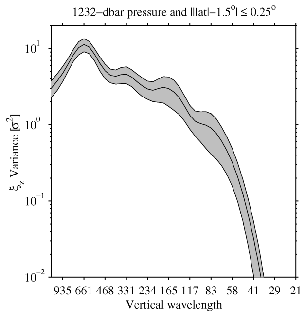
FIG. 7. Mean vertical wavelength wavelet power spectrum of \xi_z at 1232-dbar (3520 sdbar) pressure using data between 374 and 2987 dbar (1950 and 5050 sdbar) from stations within \pm 0.25^\circ of \pm 1.5^\circ from the equator (solid line). Two standard errors of the mean (shading) give roughly 95% confidence intervals, with the assumption that each CTD station is independent.
