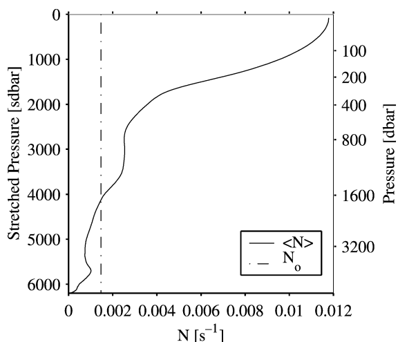
FIG. 2. The \langle N \rangle ( \text{s}^{-1} ) profile (solid line) plotted against stretched pressure (sdbar), with reference unstretched pressures (dbar) on the right-hand side; N_0 (dash-dot line) is shown for reference.
